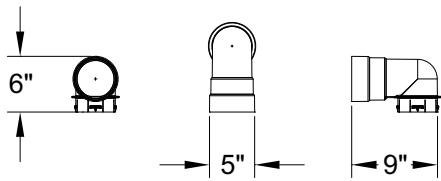
Quick4 Plus All-in-One Periscope
