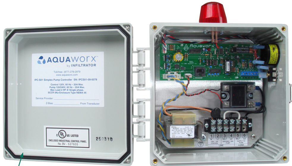
8" x 8" Enclosed
