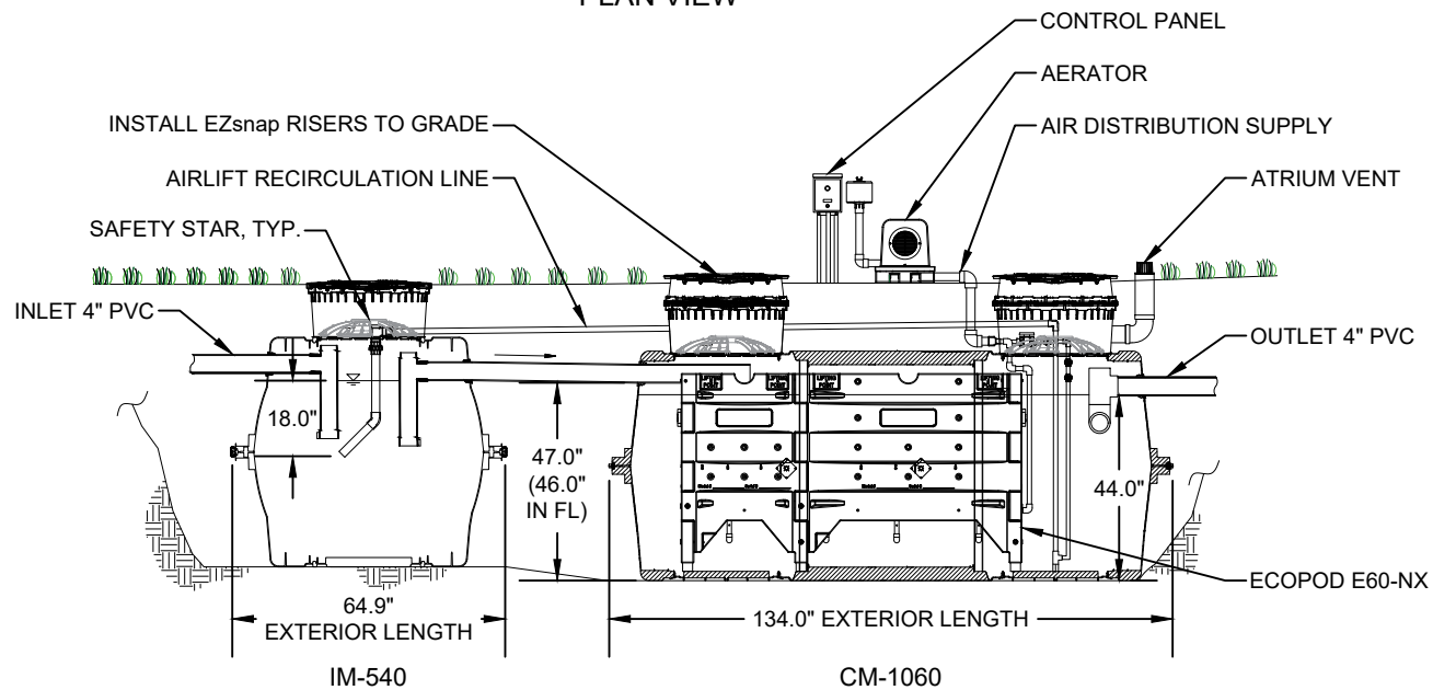
ELEVATION VIEW
