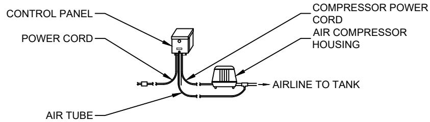
AIR COMPRESSOR HOUSING & CONTROL PANEL ASSEMBLY SCALE 1:40
