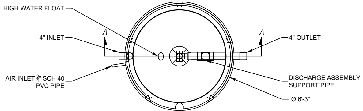
TOP VIEW DETAIL (COVER REMOVED)
