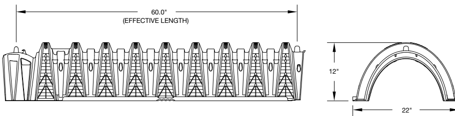
MultiPort EndCap - Part Number Q4EQ36E
