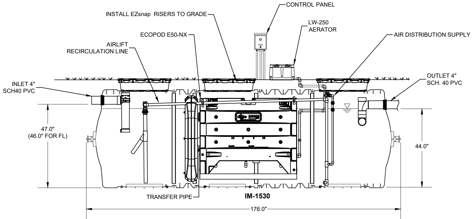
CROSS SECTION
