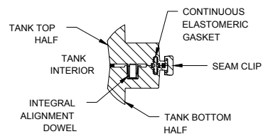
MID-HEIGHT SEAM SECTION
