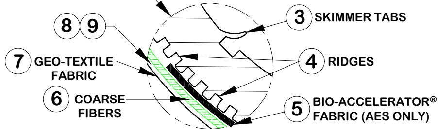
CROSS SECTION
